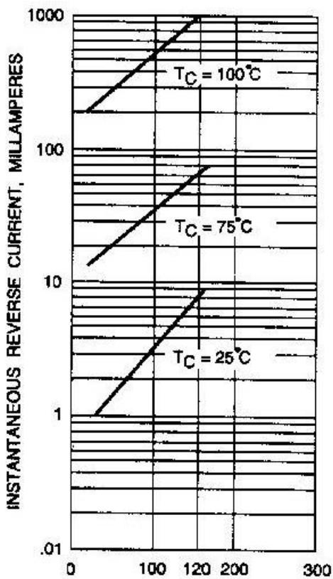
Fig. 3-TYPICAL REVERSE CHARACTERISTICS
