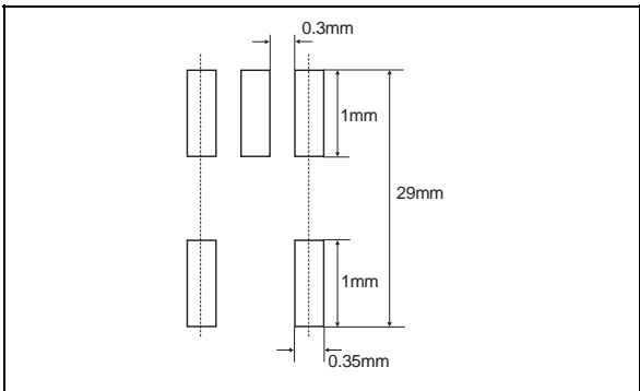
FOOT PRINT (in millimeters)
