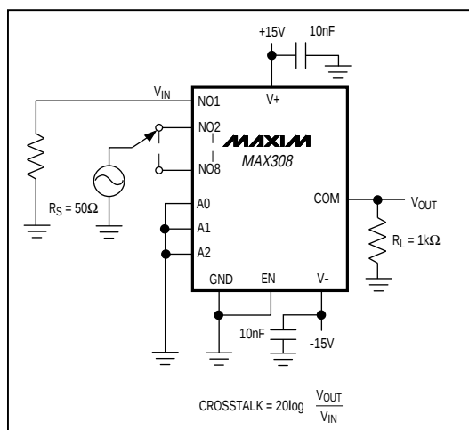
Figure 7. Crosstalk
