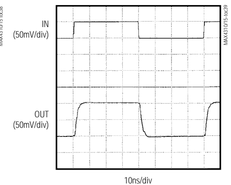
MAX4313 SMALL-SIGNAL PULSE RESPONSE
