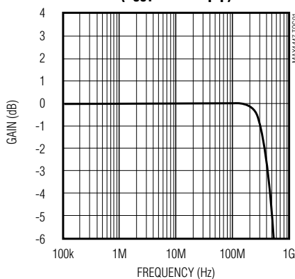
MAX4447 GAIN FLATNESS vs. FREQUENCY ( V_{OUT} = 100mVp-p )
