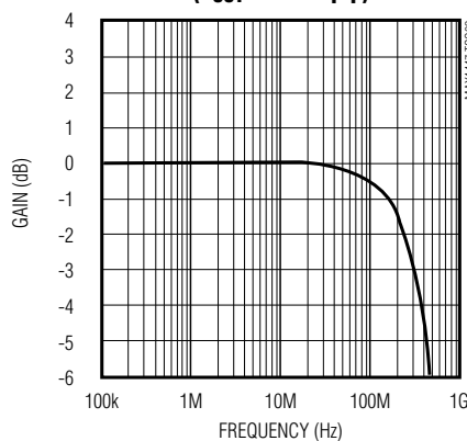
MAX4448 GAIN FLATNESS vs. FREQUENCY ( V_{OUT} = 100mVp-p )
