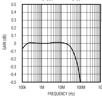
MAX4448 LARGE-SIGNAL GAIN vs. FREQUENCY ( V_{OUT} = 2Vp-p )
