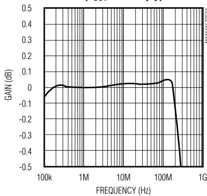
MAX4447 LARGE-SIGNAL GAIN vs. FREQUENCY ( V_{OUT} = 2Vp-p )
