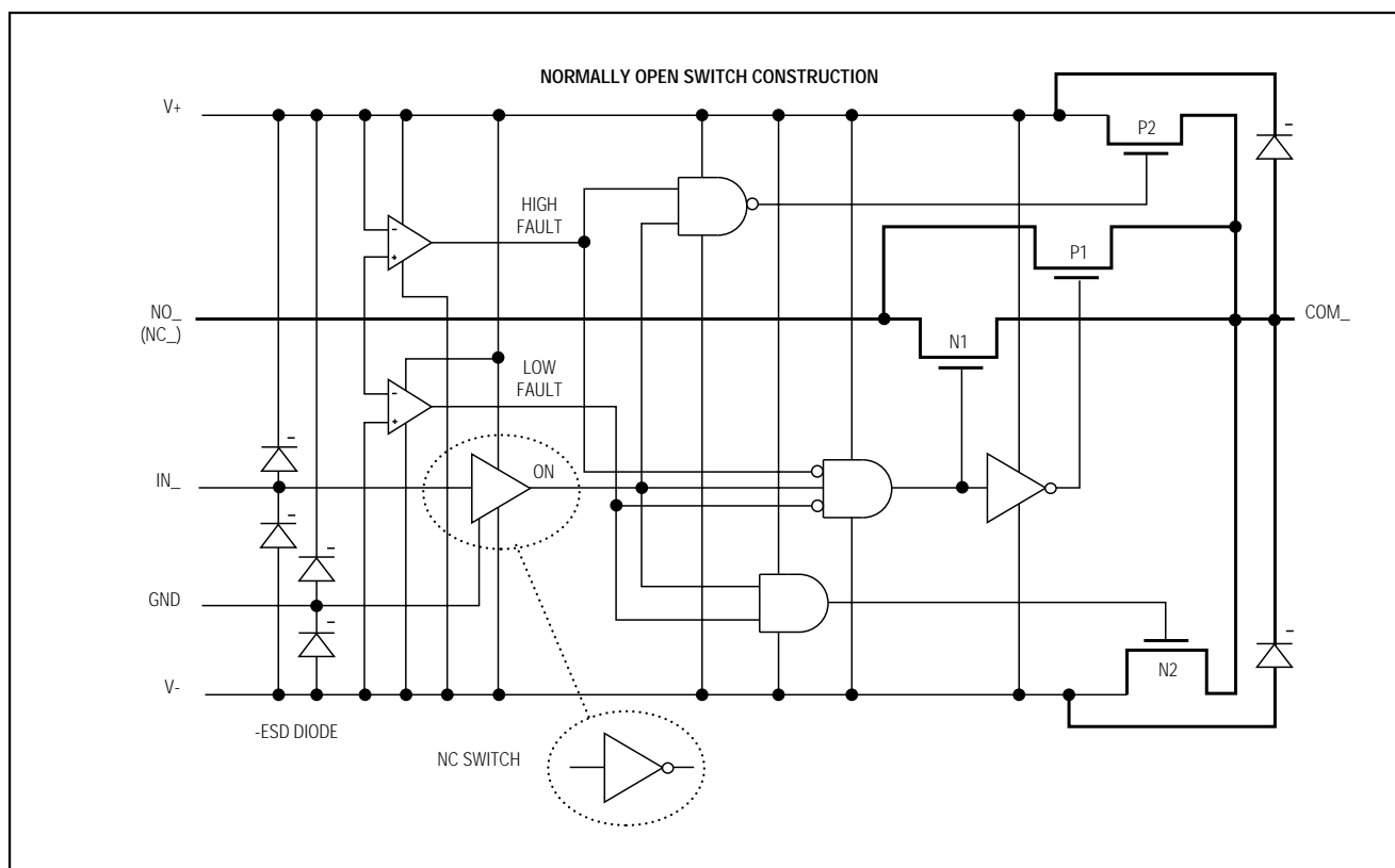
Figure 1. Block Diagram
