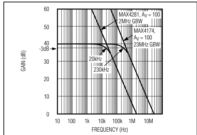
Figure 2. Gain-Bandwidth Comparison
