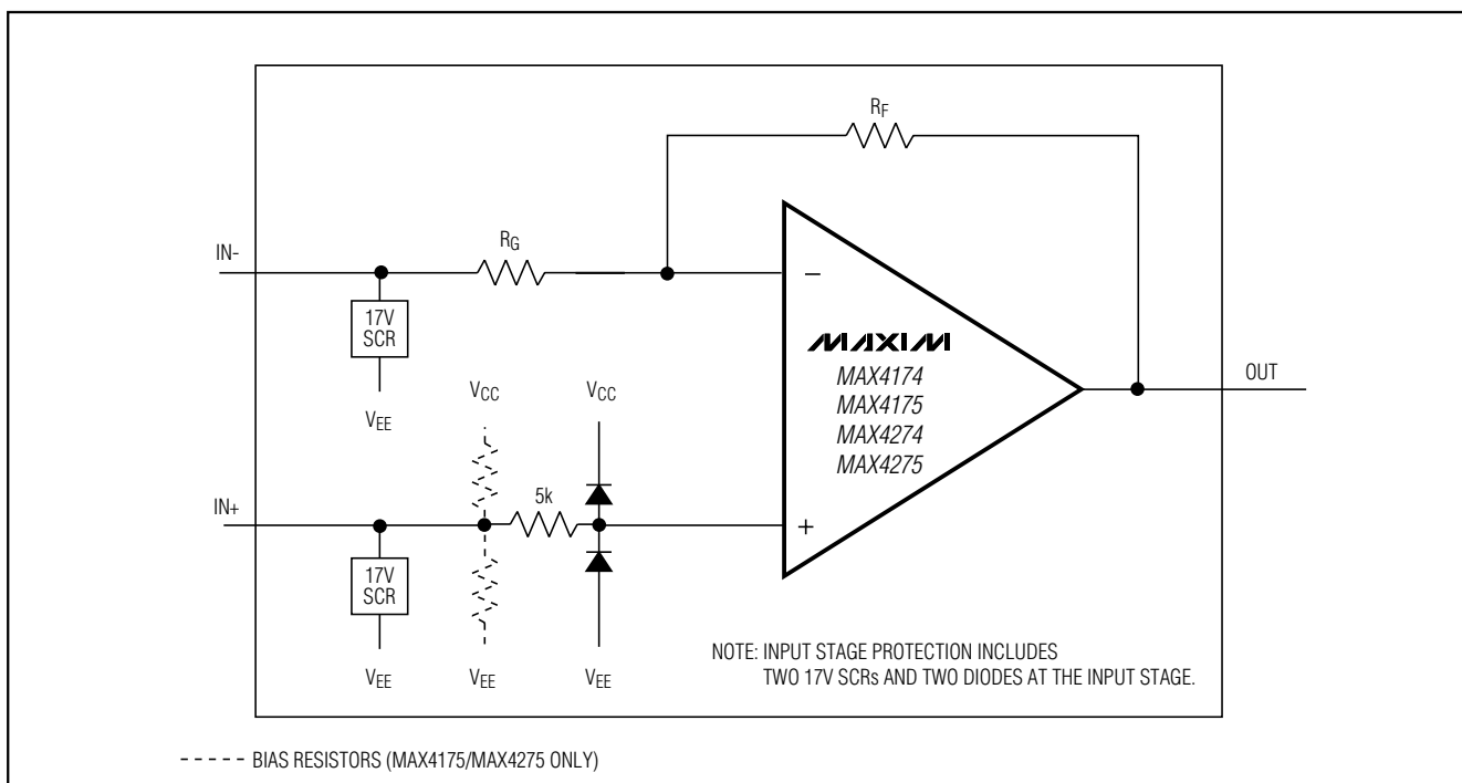
Figure 3. Input Protection
