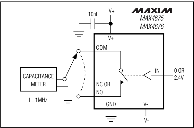
Figure 5. Channel On/Off-Capacitance
