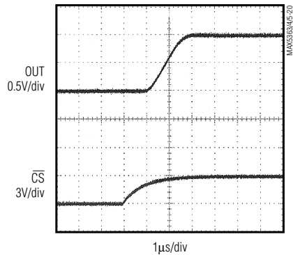
MAX5363 OUTPUT SETTLING FROM 1/4FS TO 3/4FS
