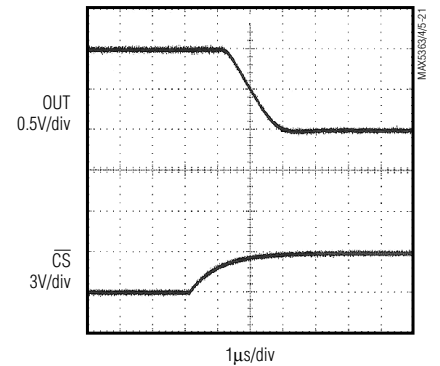
MAX5363 OUTPUT SETTLING FROM 3/4FS TO 1/4FS
