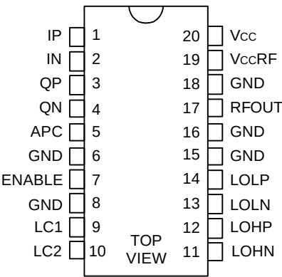
Figure 2. Pin Configuration
