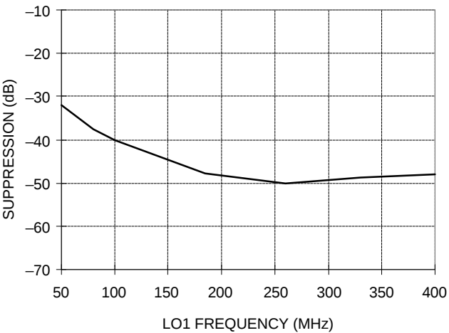
Figure 7. Carrier Suppression vs. LO1 Frequency
