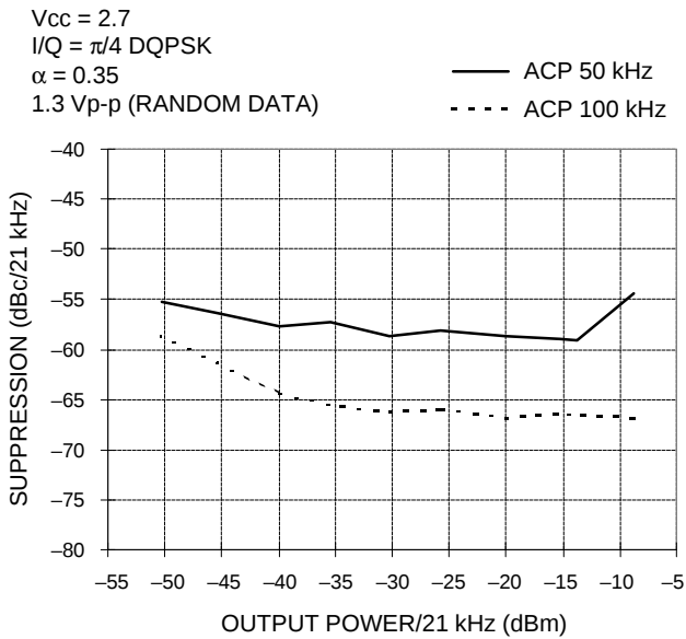
Figure 9. Adjacent Channel Suppression for PDC vs. 940 MHz Output Power
