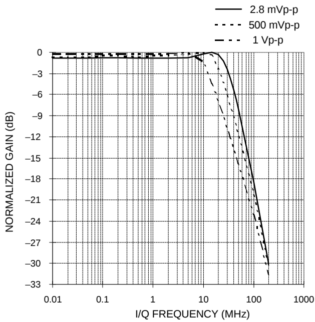
Figure 10. IQ Bandwidth vs. ac Input Voltage
