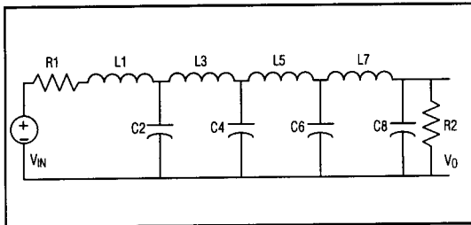
Figure 2. 8th-Order Ladder Filter Network
