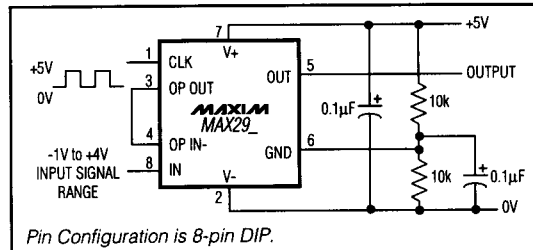
Figure 3. +5V Single-Supply Operation
