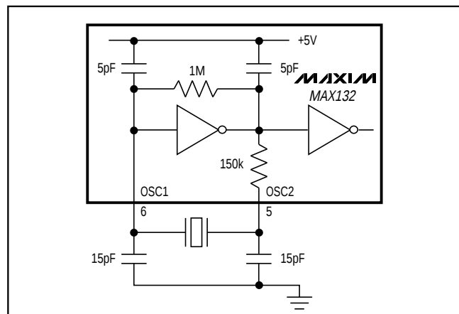
Figure 8. MAX132 Internal Oscillator Drive Circuitry
