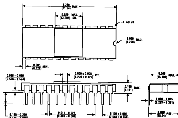
24 Lead Ceramic Sidebraz (DG)
