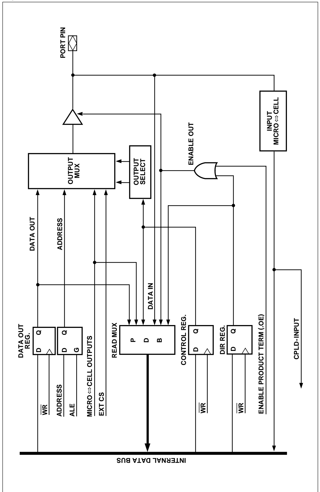
Figure 24. General I/O Port Architecture
