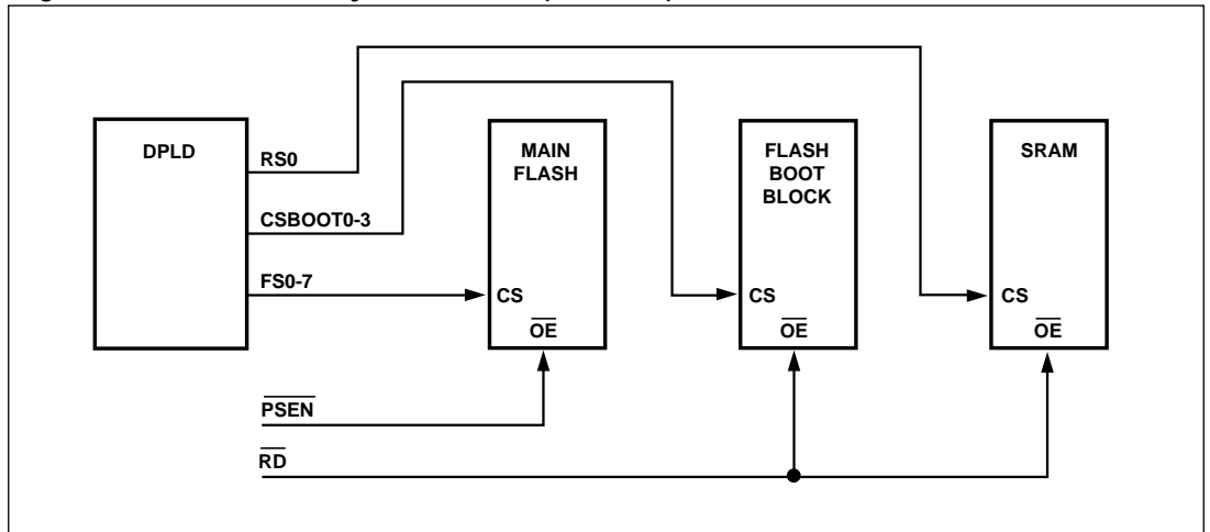
Figure 7. 80C51 Memory Modes – Separate Space Mode
