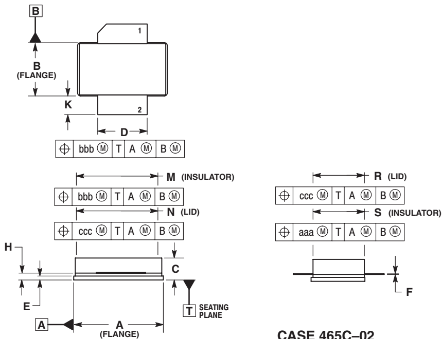
CASE 465C-02 ISSUE A (NI-880S) (MRF19090S)
