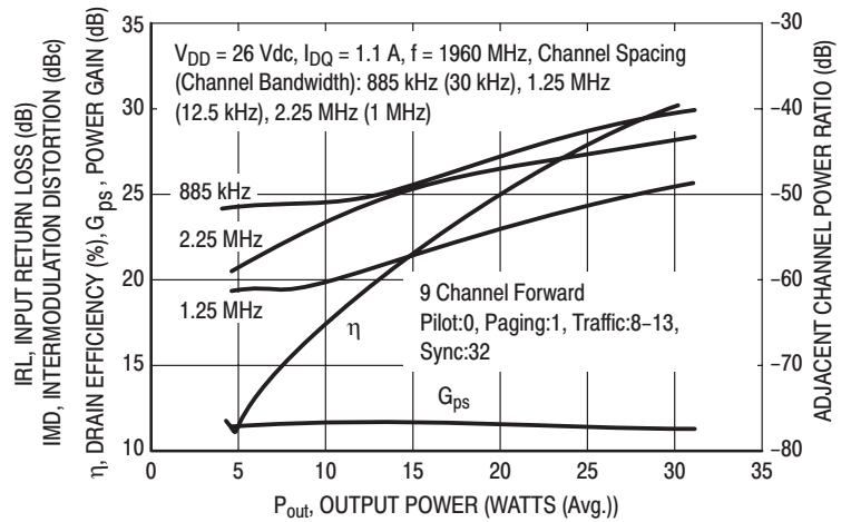
Figure 4. CDMA Performance ACPR, Gain and Drain Efficiency versus Output Power
