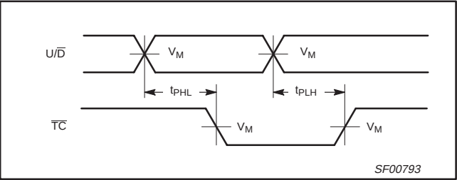
Waveform 3. Propagation Delay, Up/Down Count Control Input to Terminal Count Output
