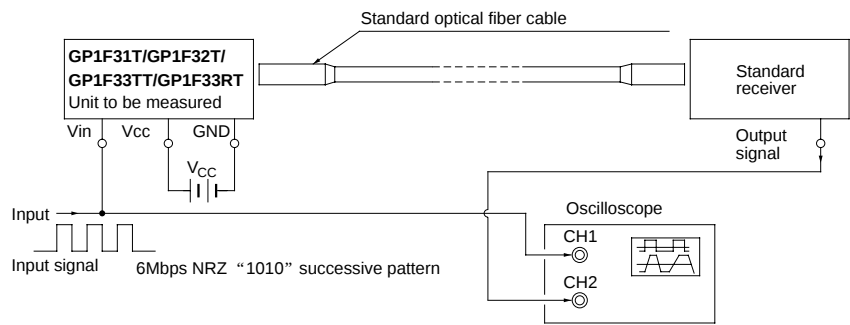
*9 Pulse response measuring method
