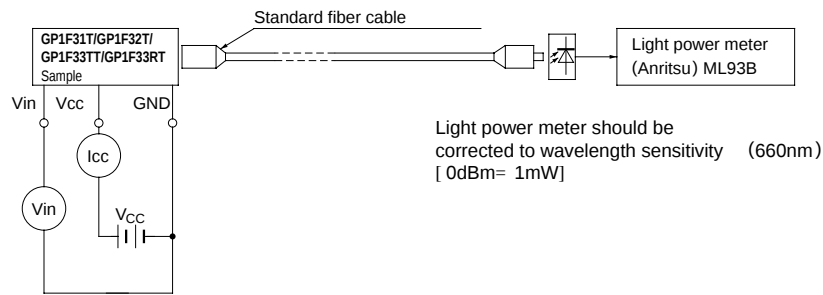
*8 Input voltage/power dissipation measuring method
