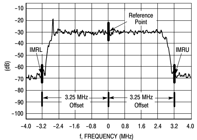
Figure 18. ATSC 8VSB Spectrum
