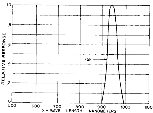
Fig. 5. Spectral Response
