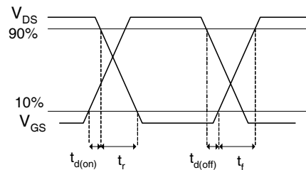
Fig 19b. Switching Time Waveforms
