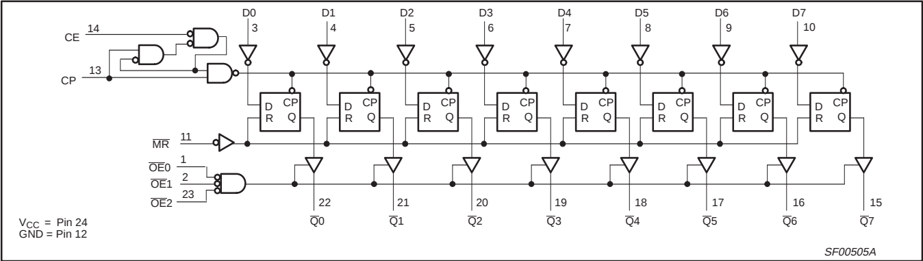
LOGIC DIAGRAM FOR 74F826
