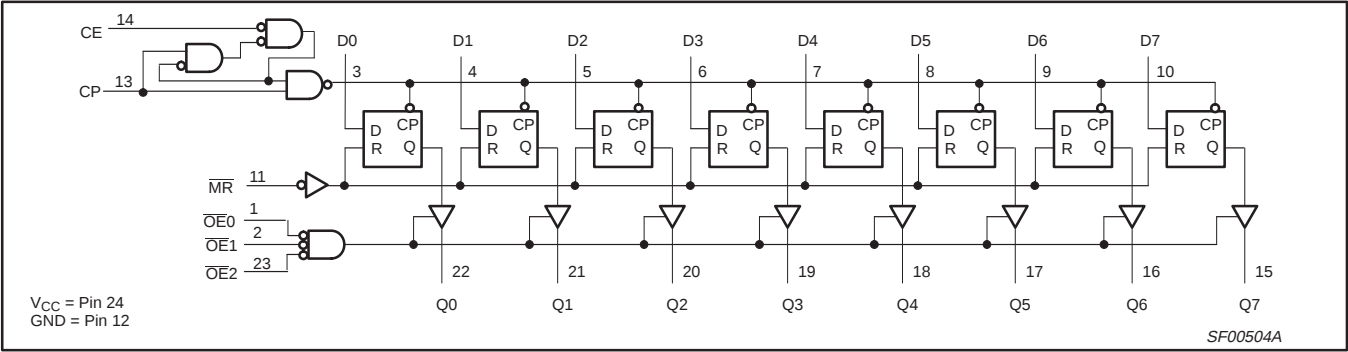
LOGIC DIAGRAM FOR 74F825
