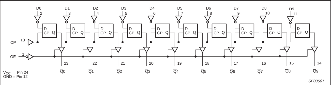
LOGIC DIAGRAM FOR 74F822
