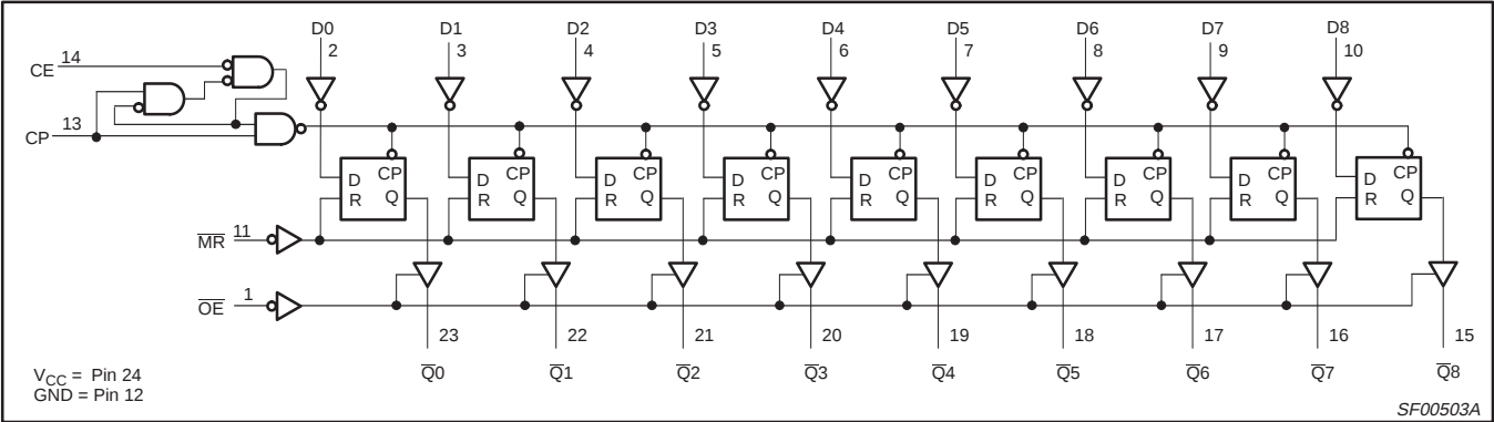
LOGIC DIAGRAM FOR 74F824
