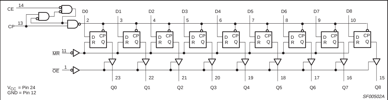
LOGIC DIAGRAM FOR 74F823
