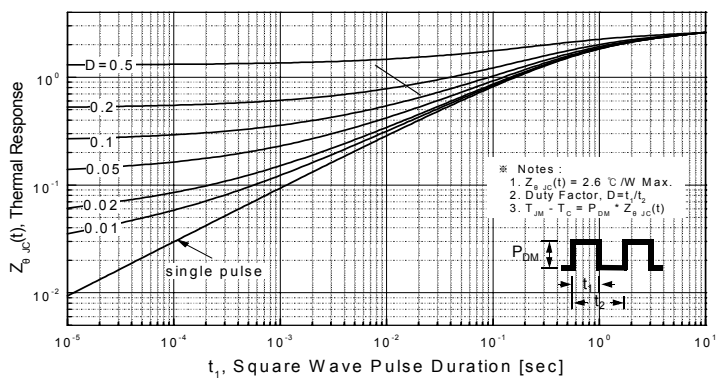
Figure 11-2. Transient Thermal Response Curve for FQP8N60C
