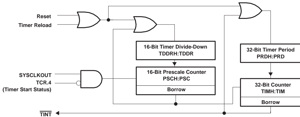
Figure 4–1. CPU-Timers
