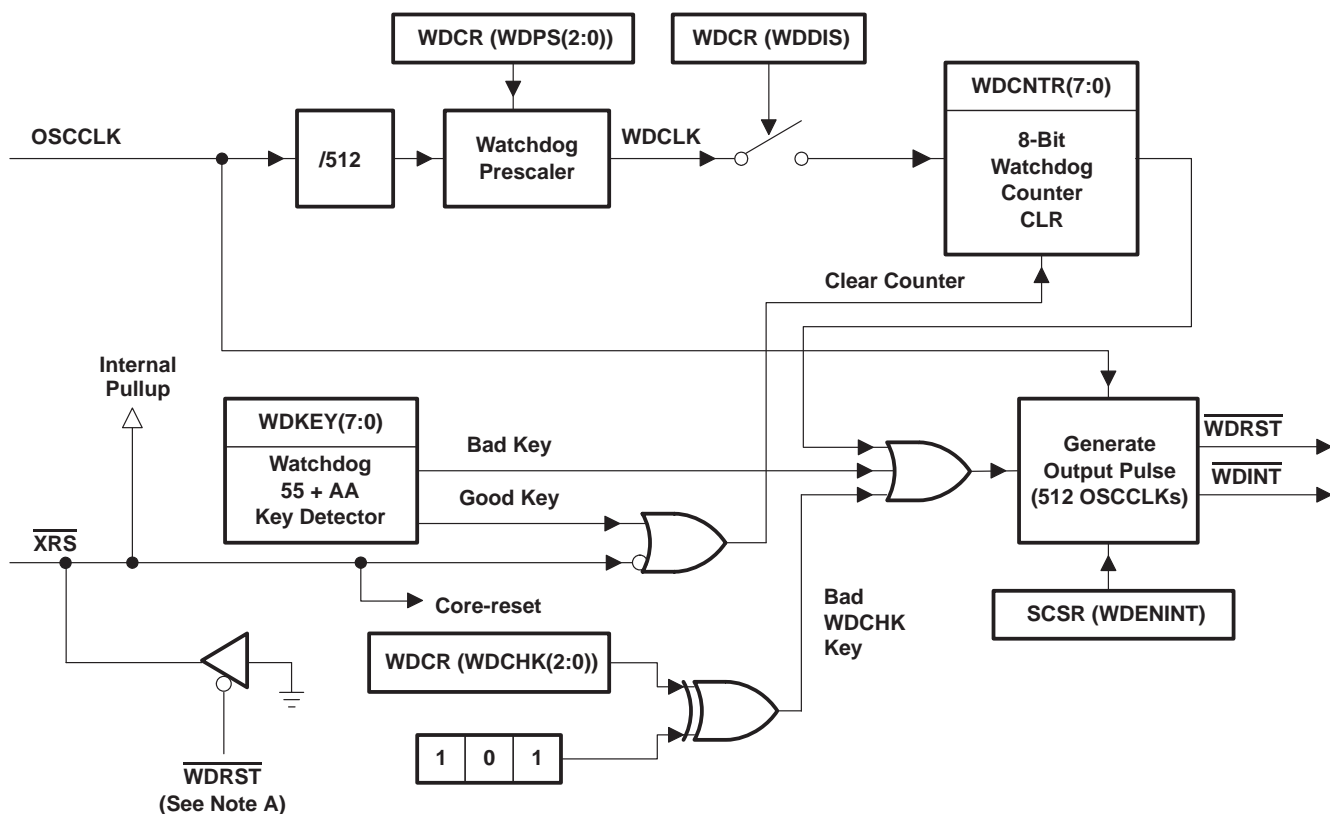
Figure 3–11. Watchdog Module
