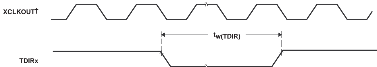
Figure 6–17. TDIRx Timing
