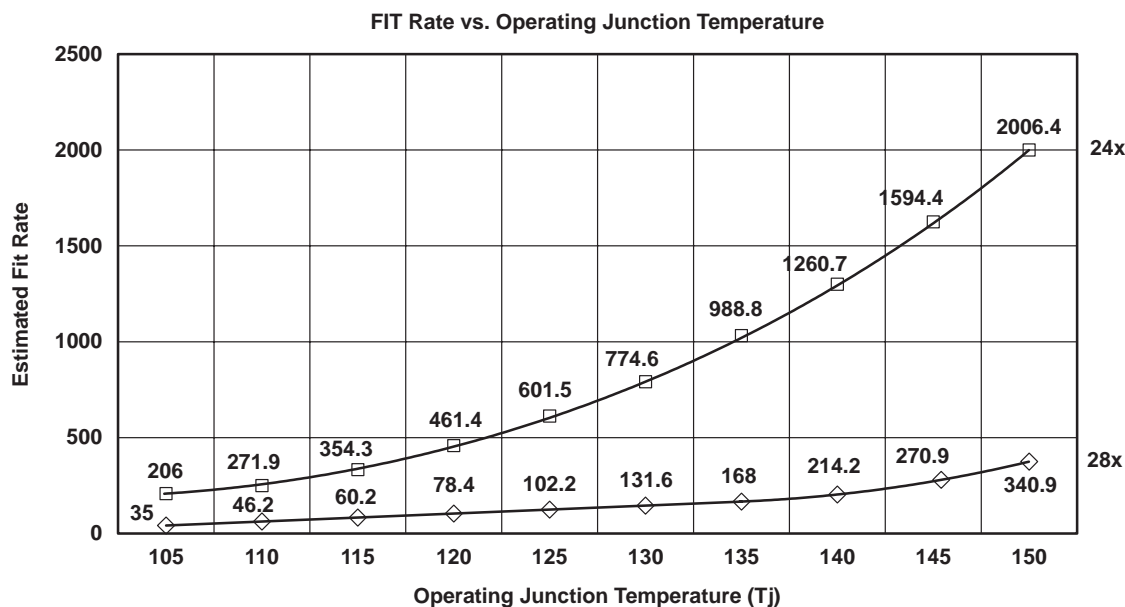
Figure 6–1. FIT Rate vs Operating Junction Temperature
