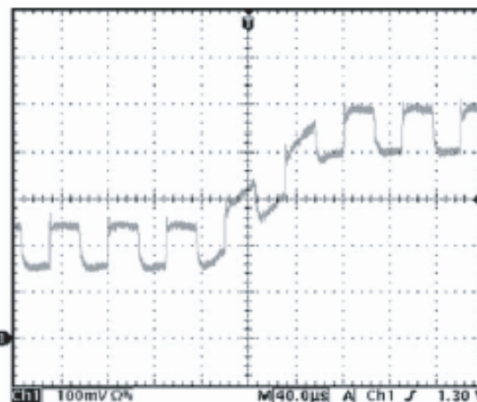
Figure 4. VID On-the-Fly Waveforms, Circuit of Figure 5, VID Change = 5mV, 5 \mu s, 50 steps, I_{OUT} Change = 5A to 65A
