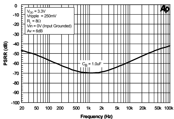
Figure 22. Power Supply Rejection Ratio
