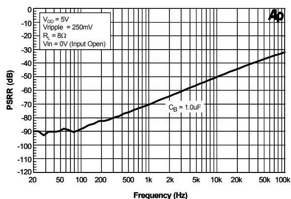
Figure 19. Power Supply Rejection Ratio
