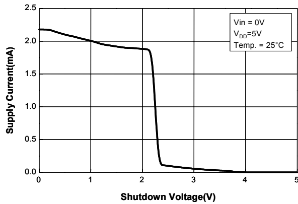
Figure 25. Supply Current vs. Shutdown Voltage
