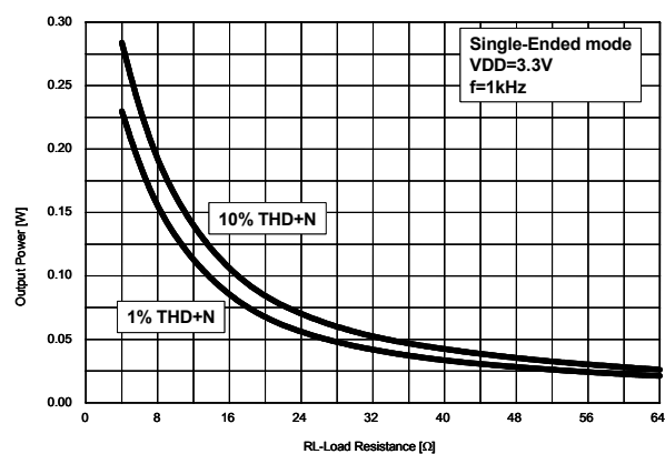
Figure 42. Output Power vs. Load Resistance
