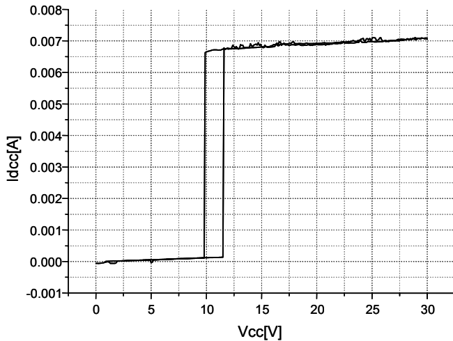
Figure 1. UVLO
