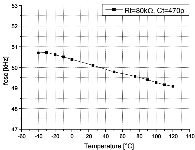
Figure 5. Switching Frequency
