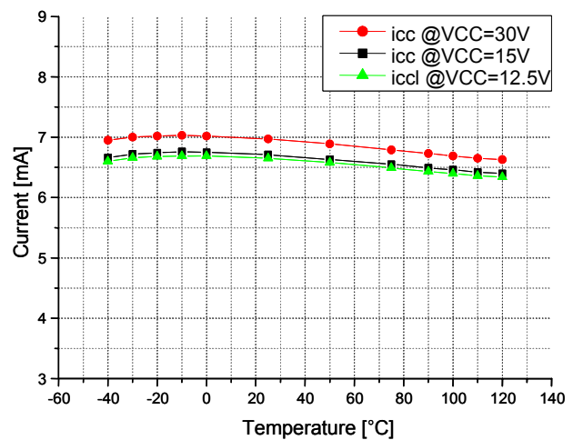
Figure 4. Operating Current
