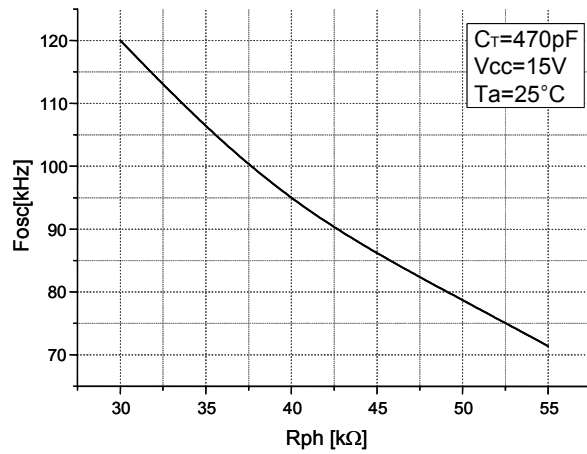
Figure 6. Preheating Frequency, C_T = 470pF
