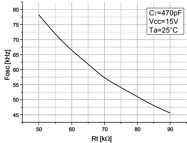
Figure 7. Switching Frequency, C_T = 470pF
