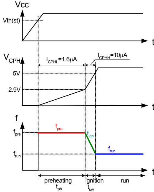
Figure 12. Timing Diagram
