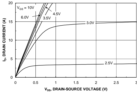
Figure 11. On-Region Characteristics.
