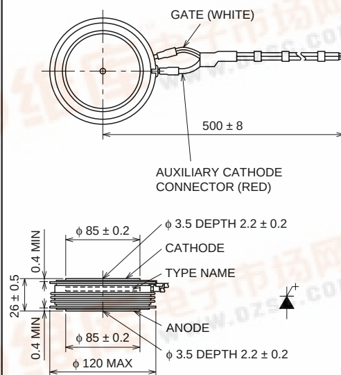
OUTLINE DRAWING
