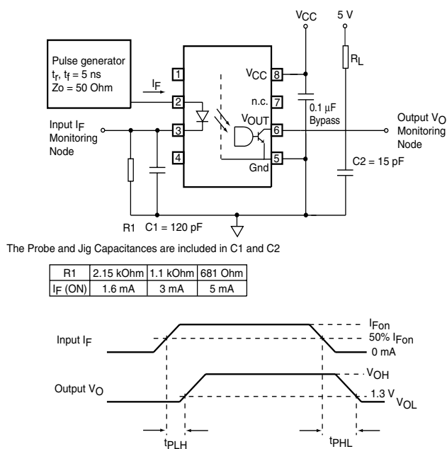
Fig. 28 Test Circuit for t_{PLH} , t_{PHL} , t_r and - SFH6705
