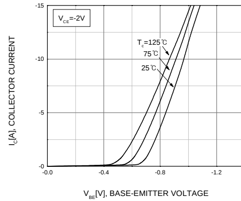
Fig. 2 Transfer Characteristic
