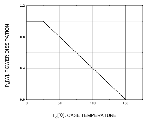
Fig. 7 Power Derating
