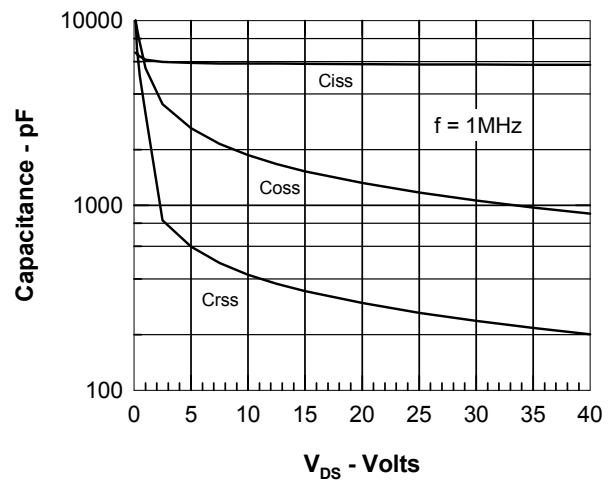
Figure 8. Capacitance Curves
