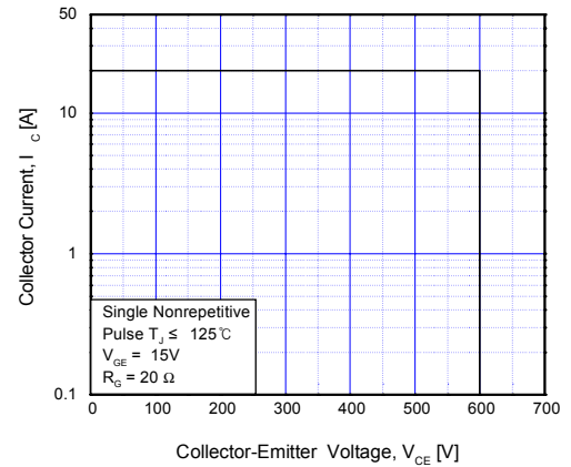
Figure 16. RBSOA Characteristics
