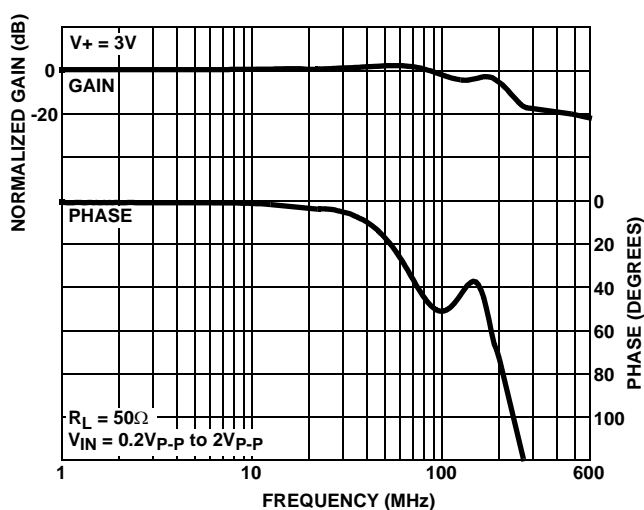
FIGURE 15. FREQUENCY RESPONSE
