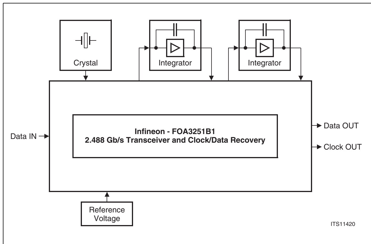
Figure 5 External Components Required for Operation of FOA3251B1
