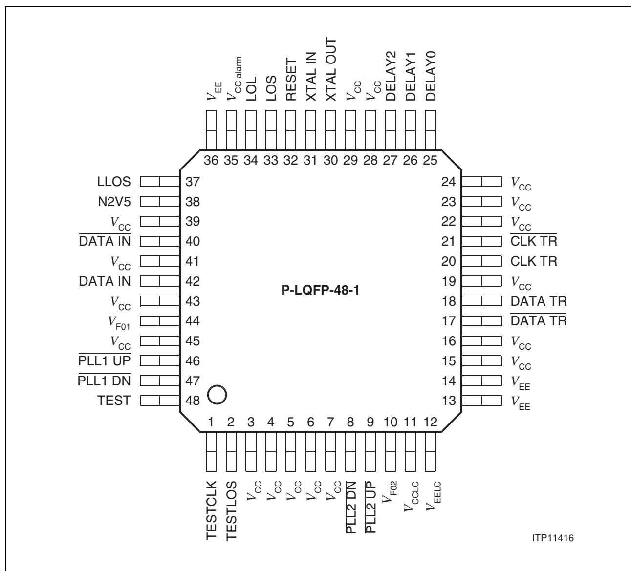
Figure 1 Pin Configuration
