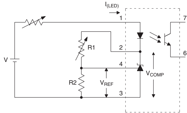
FIG. 2. \Delta V_{REF}/\Delta V_{COMP} TEST CIRCUIT
