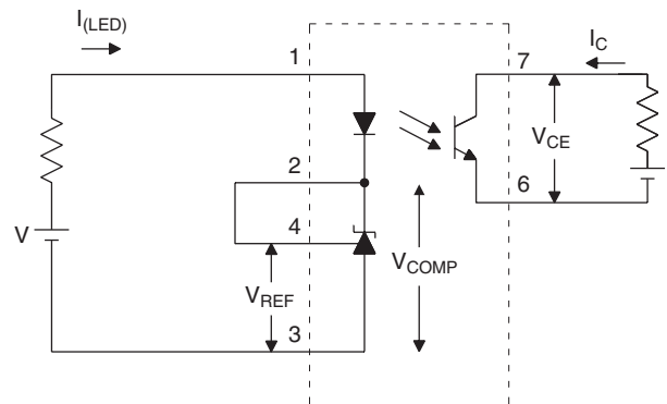
FIG. 6. CTR, V_{CE(sat)} TEST CIRCUIT
