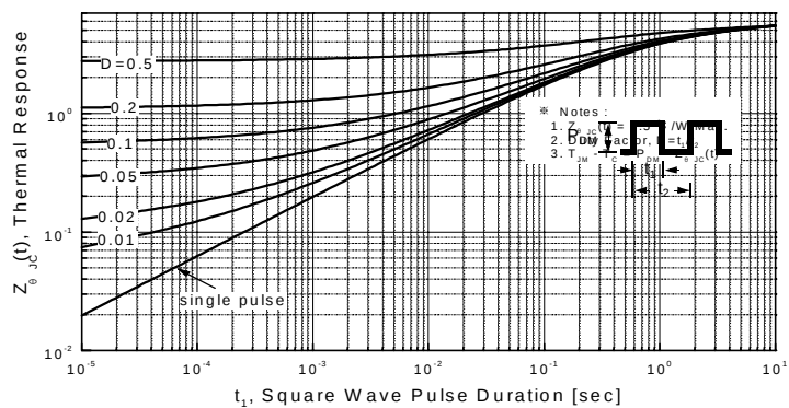
Figure 11-2. Transient Thermal Response Curve for FQPF2N60C
