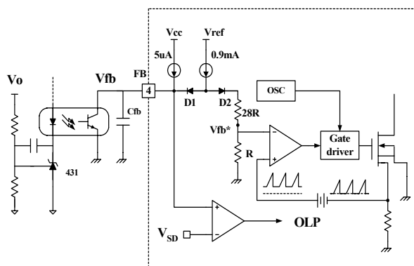
2. Feedback Control : The FS6X1220R employs current mode control. The voltage of the feedback pin is compared with the current sense voltage for pulse width modulation (PWM). Figure 2 illustrates the simplified PWM block. The feedback voltage determines the peak drain current of the SenseFET. Usually opto-coupler along with TL431 are used to implement feedback network. The collector of the opto-coupler transistor is connected to feedback pin and the emitter is connected to the ground pin. When the voltage of the reference pin of TL431 exceeds the internal reference voltage of 2.5V, the opto-coupler diode current increases, pulling down the feedback voltage.
