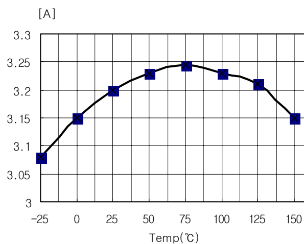
Figure 12. Peak Current Limit vs. Temp.
