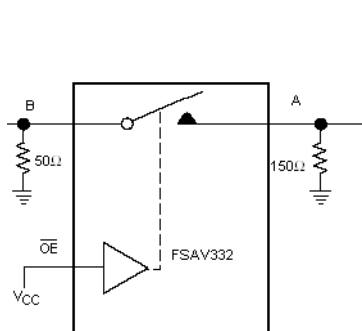
FIGURE 3. OFF Isolation Test
