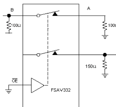
FIGURE 4. Crosstalk Test
