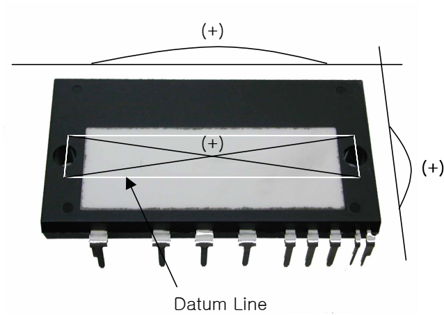
Fig. 7. Flatness Measurement Position of The Ceramic Substrate
