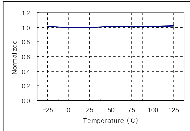
Shutdown Feedback Voltage (Vsp) vs. Ta
