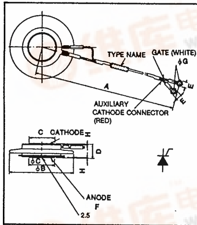
FT500AH Outline Drawing
