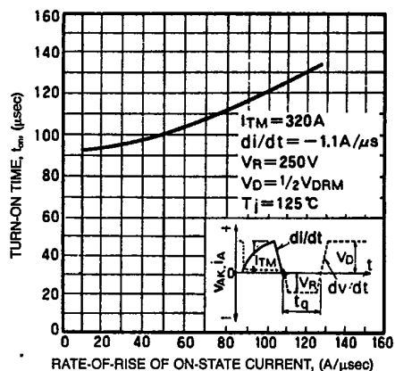
TURN-ON TIME VS. RATE-OF-RISE (TYPICAL)
