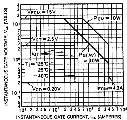
GATE CHARACTERISTICS
