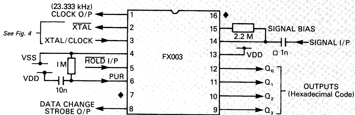
Fig. 2 Dual-In-Line
