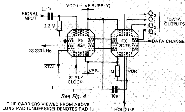
Fig. 3 Chip Carrier
