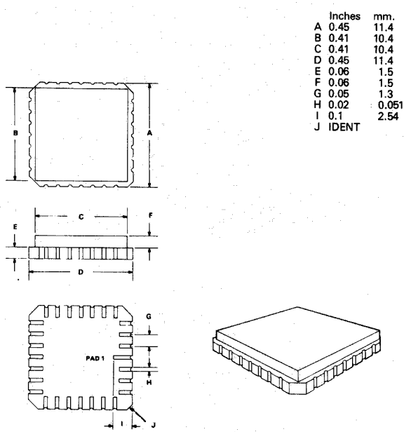
Fig. 7 FX102K/202*K Chip Carrier Package
