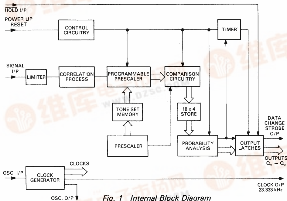
Fig. 1 Internal Block Diagram
