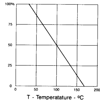
FIGURE 3 DERATING CURVE
