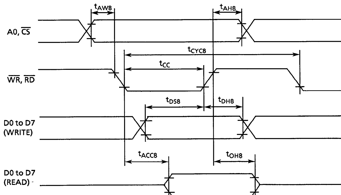
Timing Chart
