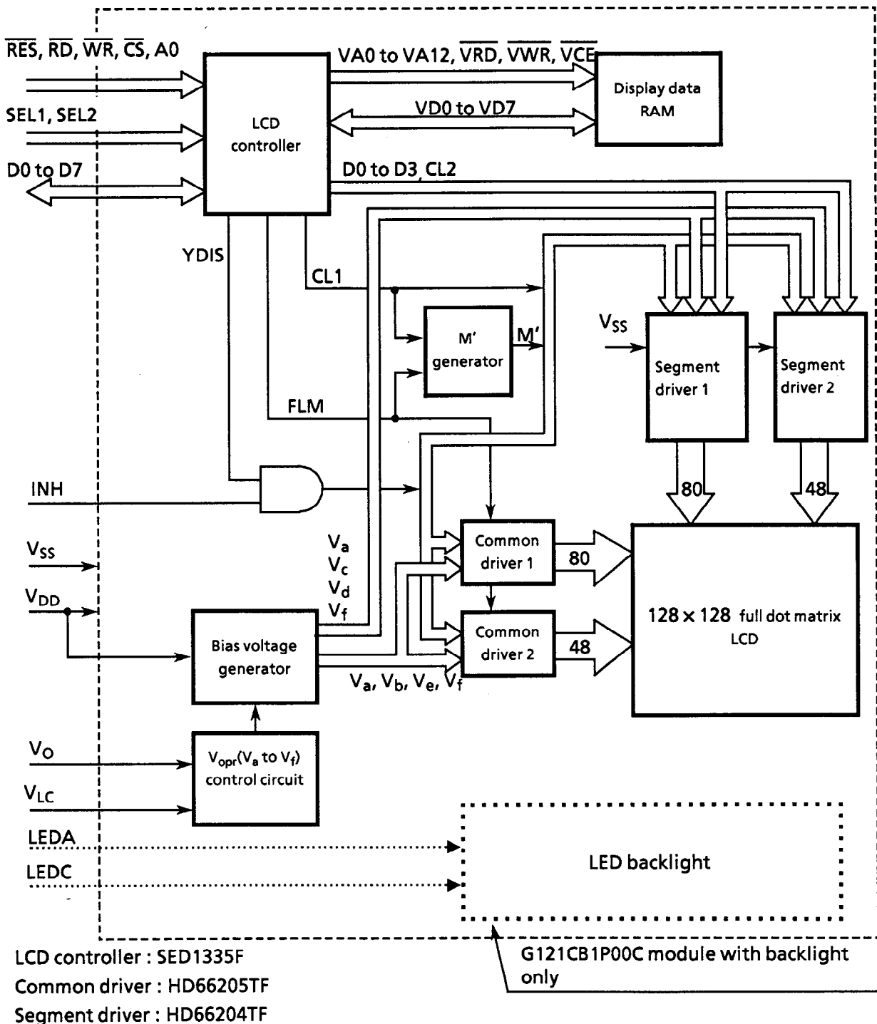
Figure 3 Block Diagram
