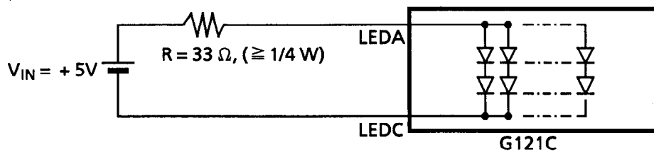
Figure 14 LED Backlight Driver Example 1
