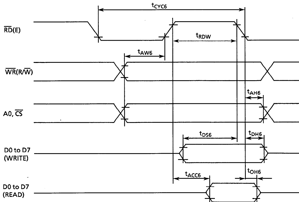
Timing Chart
