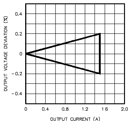
FIGURE 4. * OUTPUT VOLTAGE DEVIATION VS. OUTPUT CURRENT
