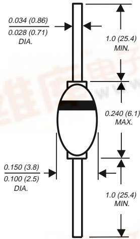
DO-204AP
