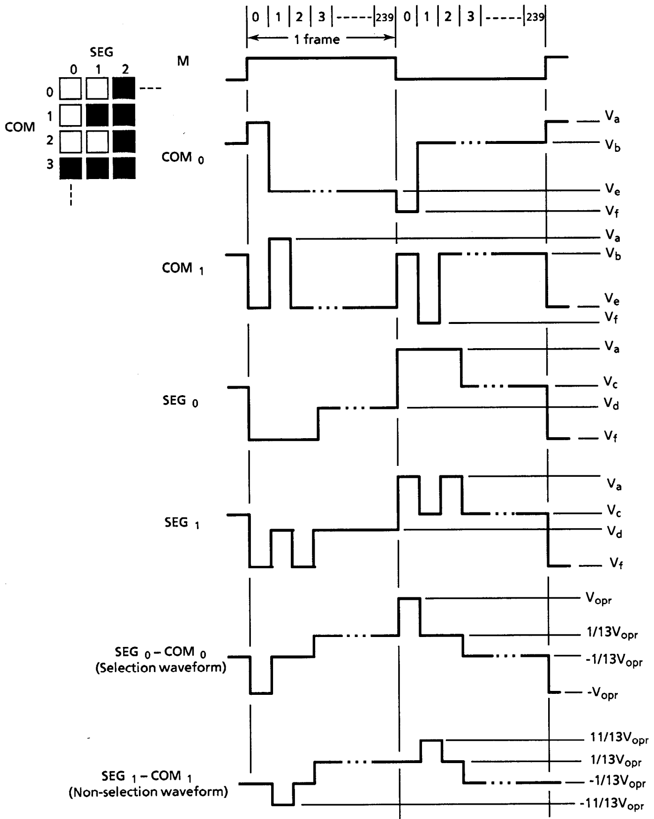
Figure 2 Drive Waveform
