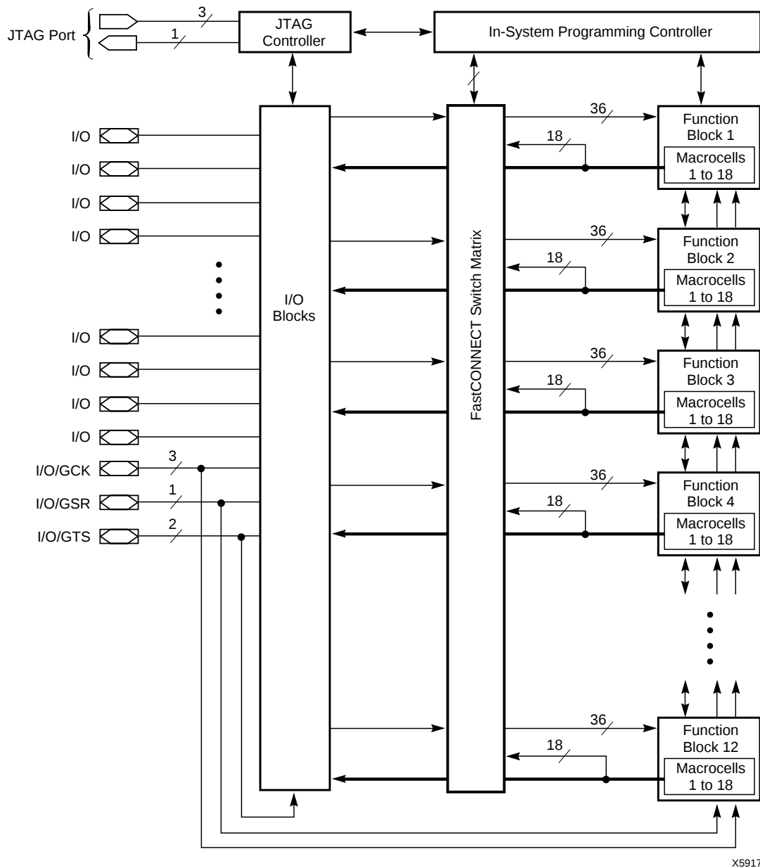
Figure 2: XC95216 Architecture
